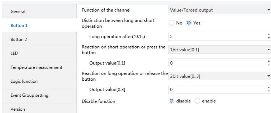
Fig. 4.4 Parameter Setting Page “Button x- Value/Forced output”
