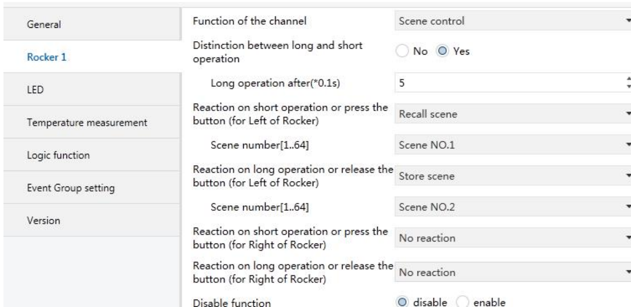
Fig. 4.13 Parameter Setting Page “Button x- Scene control”
